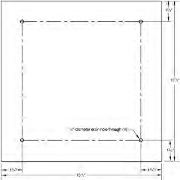
(Top/Bottom pattern from combined halves of split plan)
