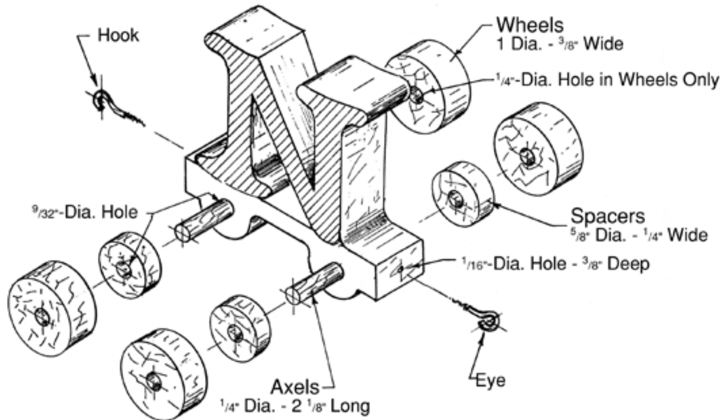
Car Assembly Drawing
